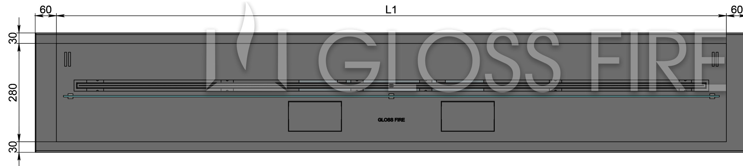
Top view
